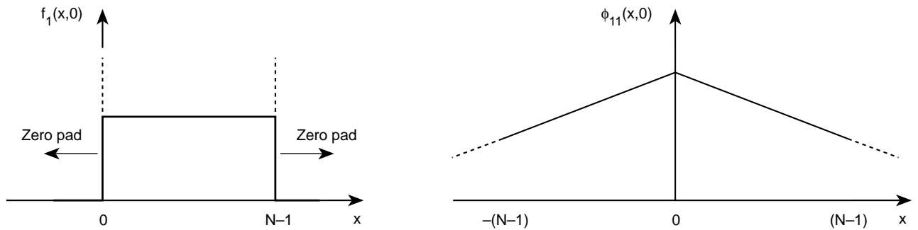
FIG. 8 Effect of zero padding in the evaluation of the autocorrelation function (ACF) showing uniform image data and the corresponding ACF in one dimension.
